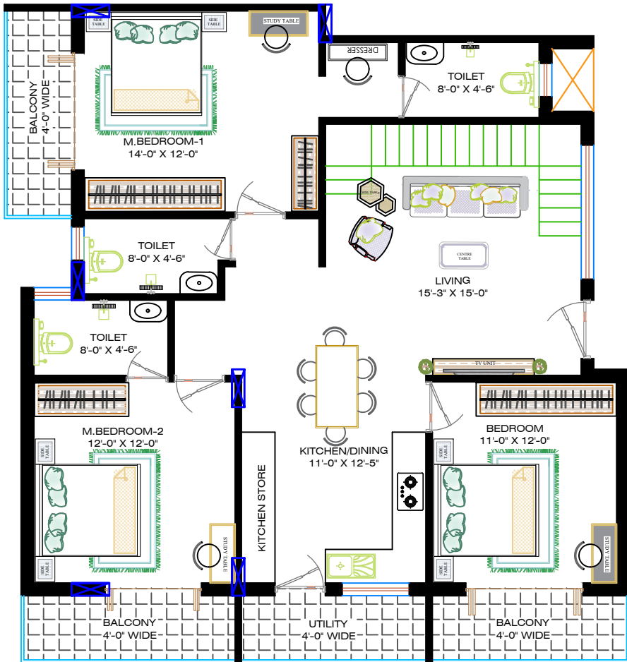
FLOOR PLAN
